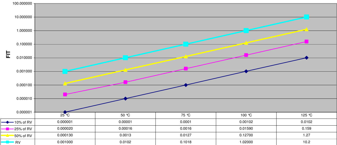
NPO failure rates at 90% confidence
